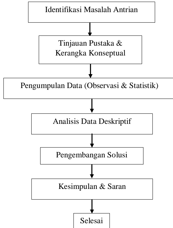
Gambar III. 1 Tahapan Penelitian
